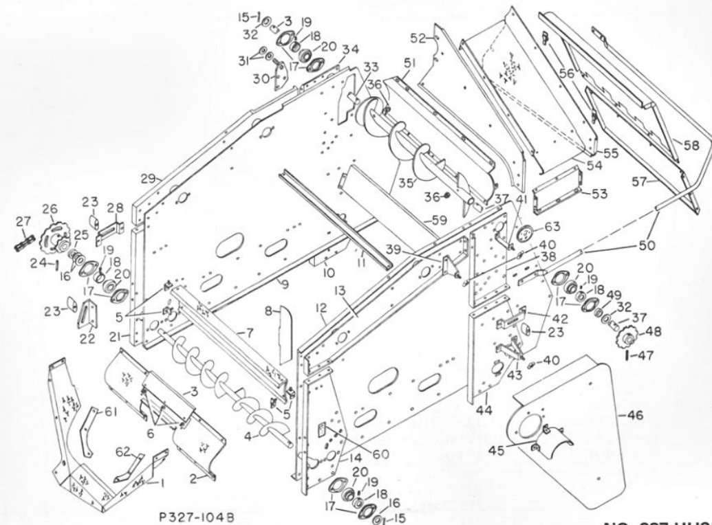
NO. 327 HUSKING UNIT LOT P272 -
