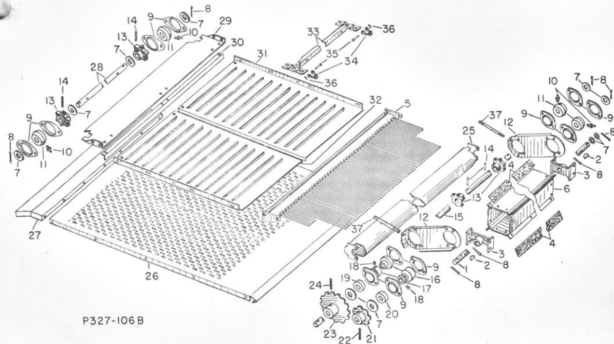
NO. 327 HUSKING UNIT LOT P272 -
